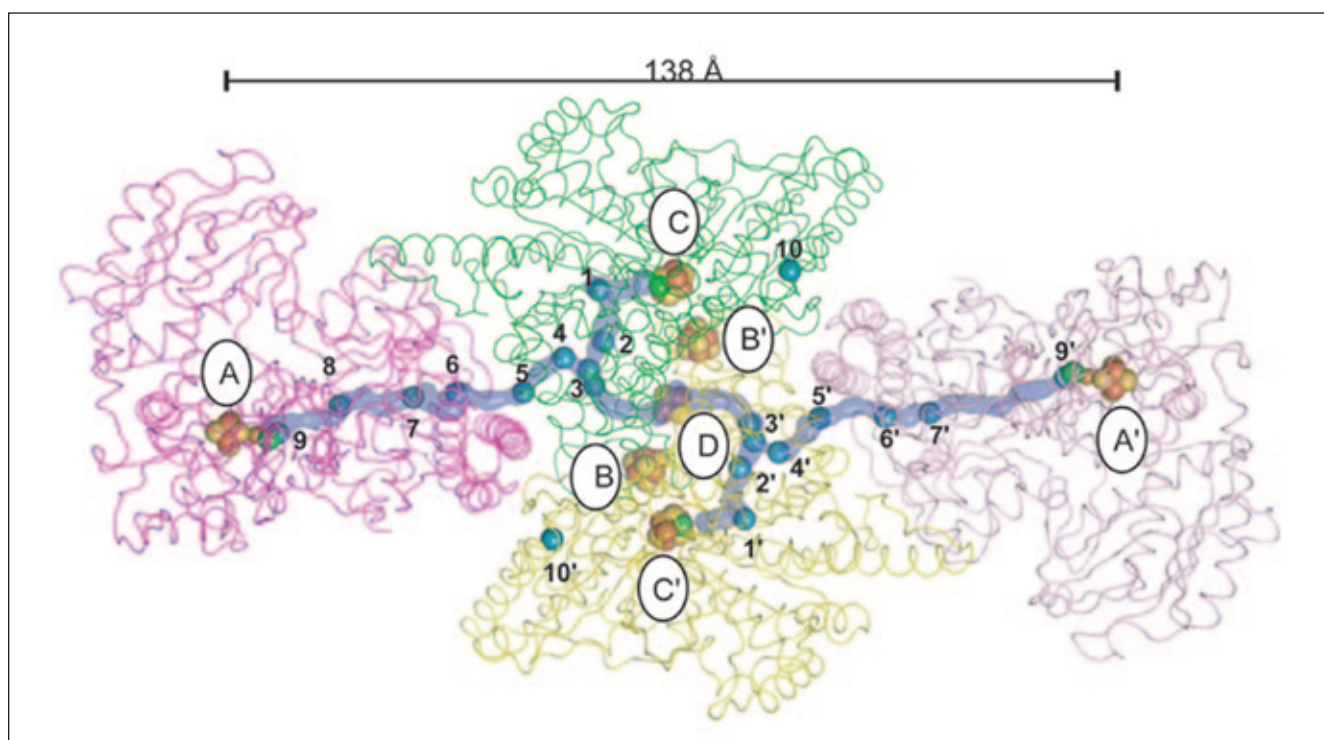
A gas channel between the active sites of CO dehydrogenase (C) and acetyl-CoA synthase (A). Ragsdale is studying this enzyme complex, which is responsible for reductive conversion of \text{CO}_2 to acetyl-CoA. Revised from Doukov, T. I., et al. (2008). Biochem. 47 , 3474-3483.
